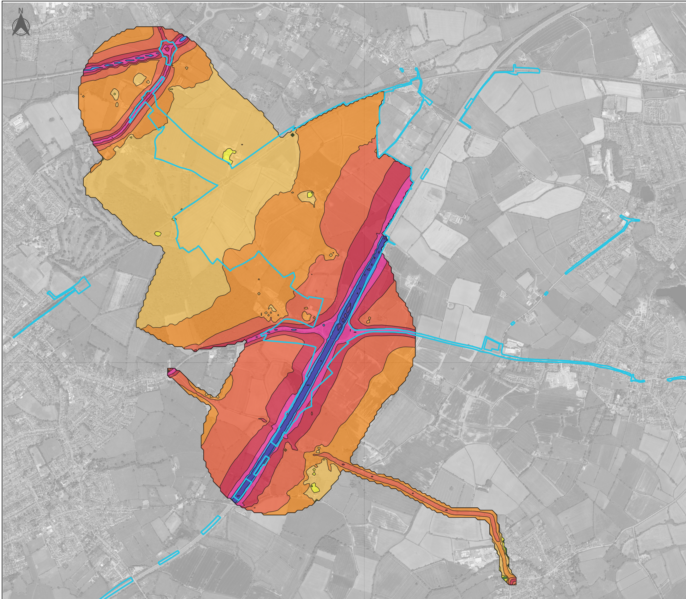
Figure 10.4 - Short-term Development Generated Road Traffic Assessment without Mitigation - Noise Contours 'without development' dB LA10, 18hr
